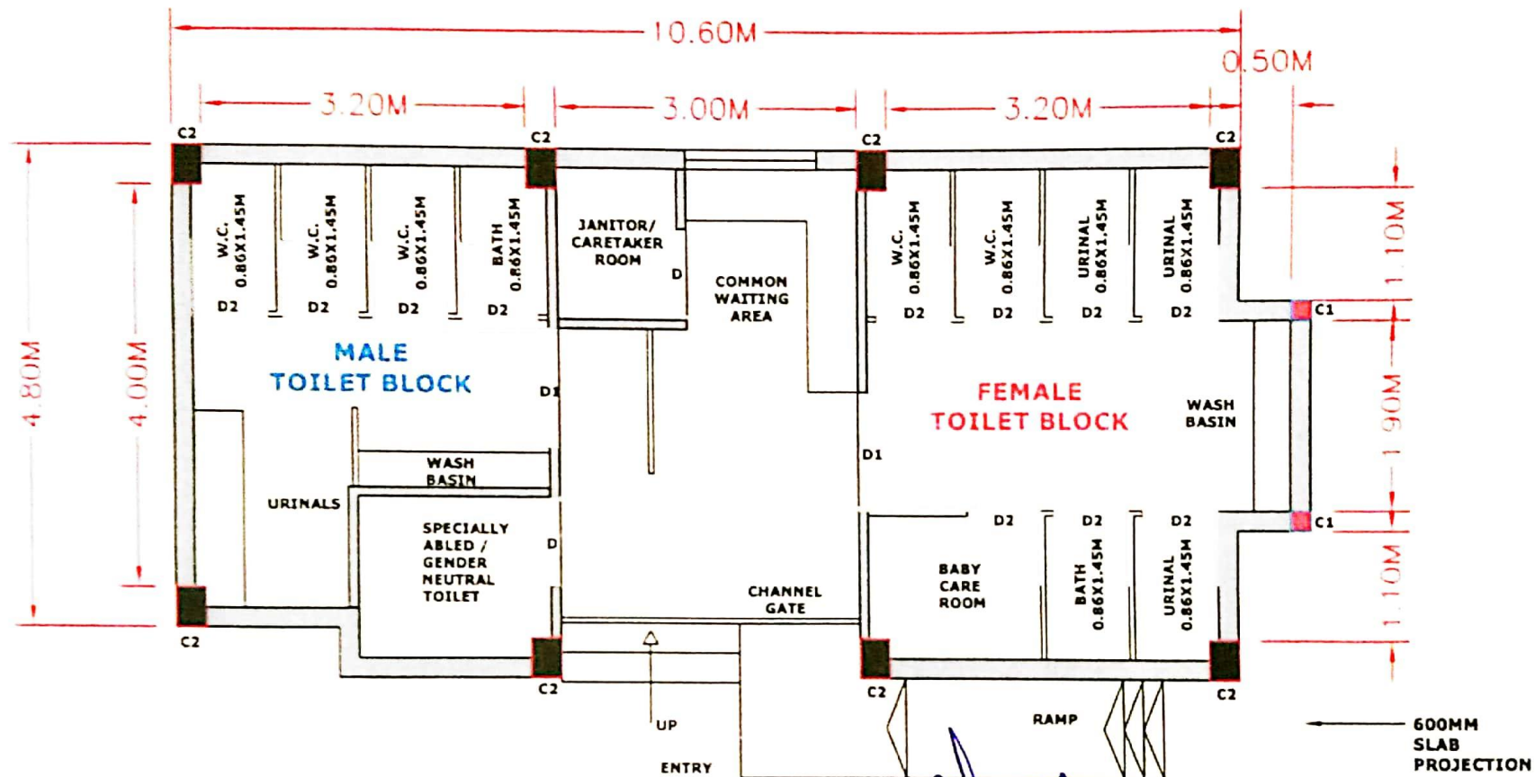
PLAN
